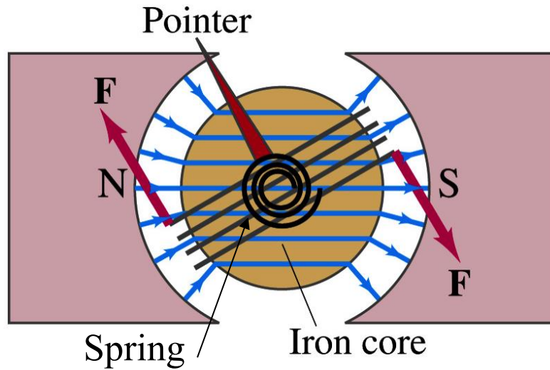
Galvanometer (electric current measurement)
