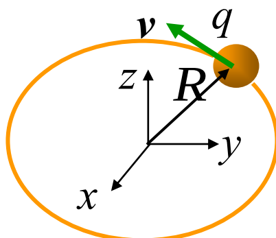
(moving charge on a circular path)
