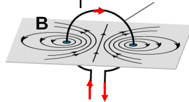
"Infinite" wire
