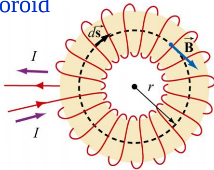
Toroid
