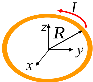
Ampere model (current in circular turn)
